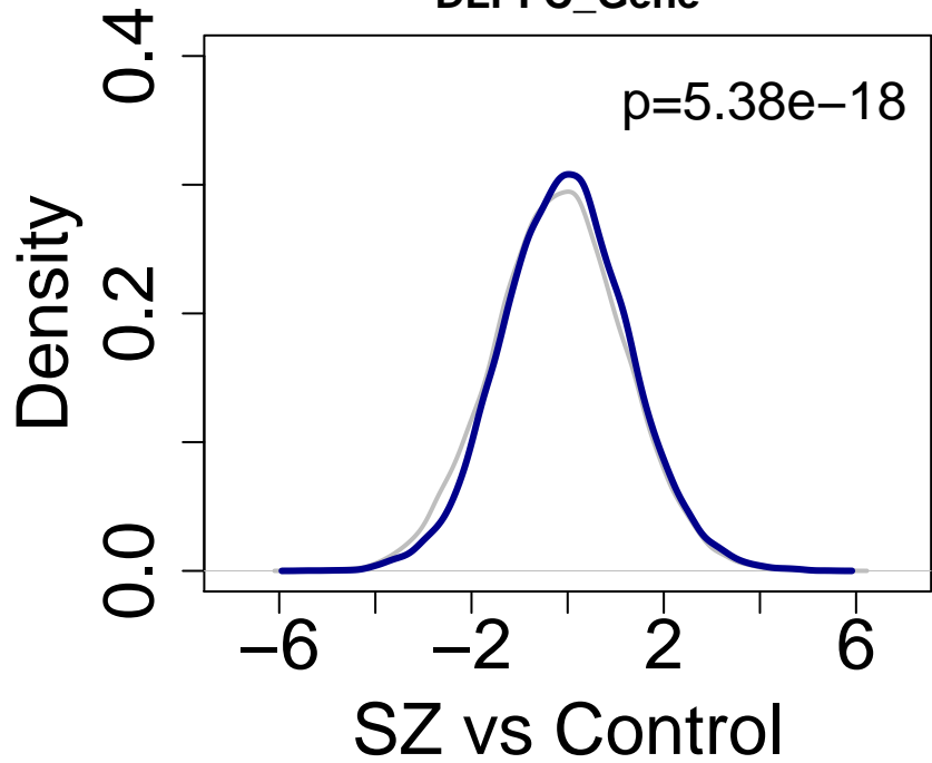
DLPFC_Gene
