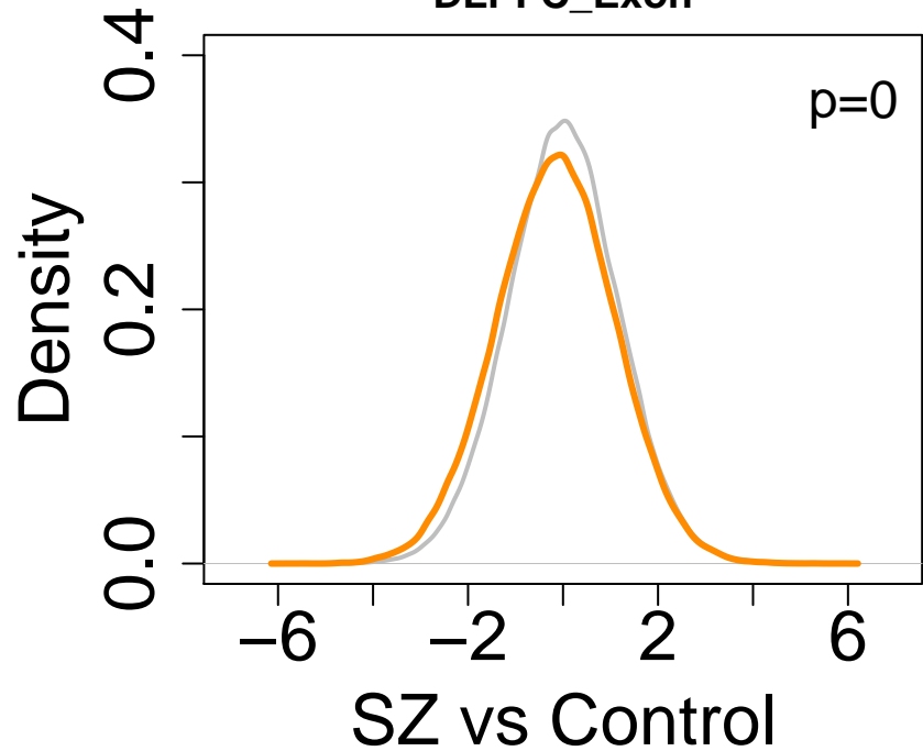
DLPFC_Exon
