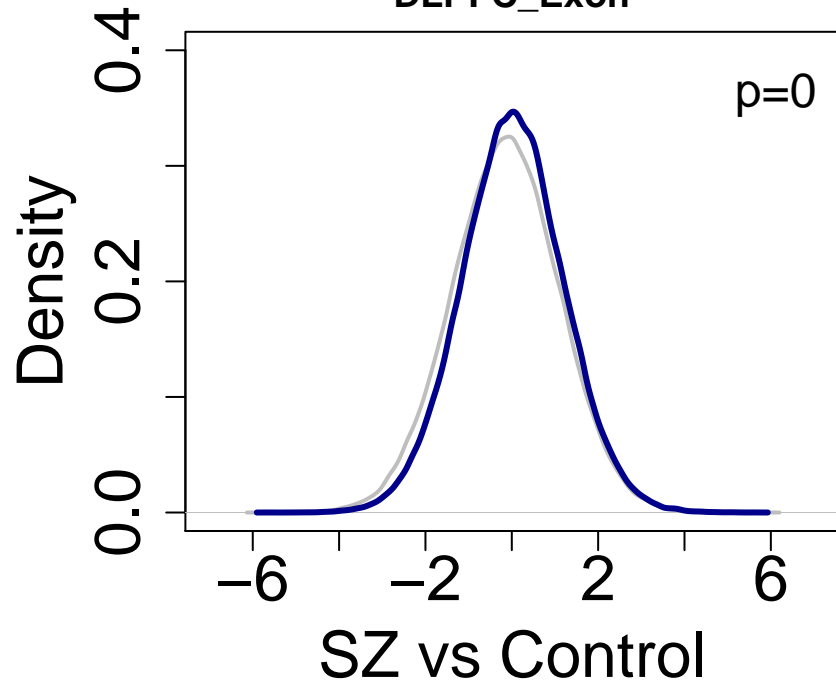
DLPFC_Exon
