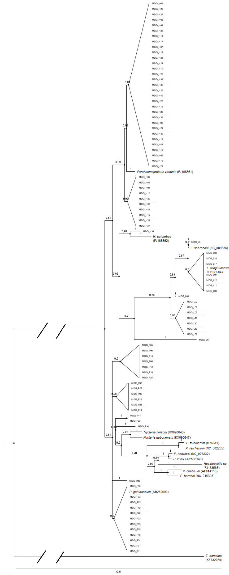
Figure S1: Detailed Bayesian phylogeny.
